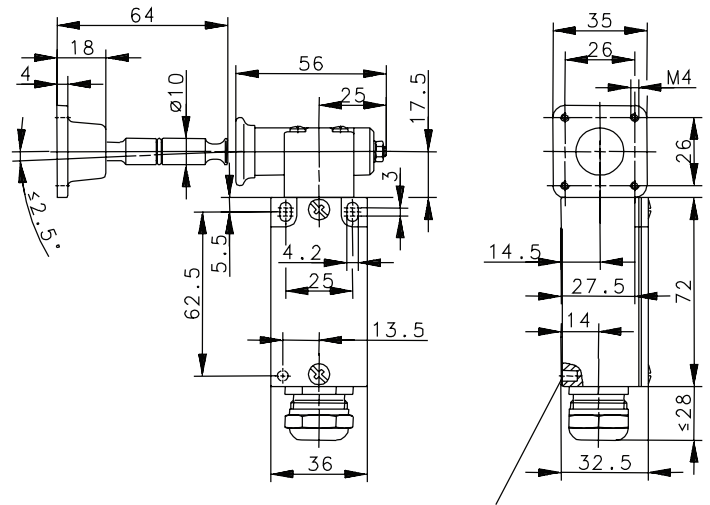
Blind hole for fitted pin Ø4 ; 5.5 deep
