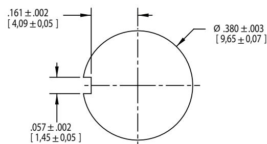
Suggested Mounting Panel Cutout
