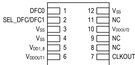
2.5 × 2.5 mm 12-DFN
