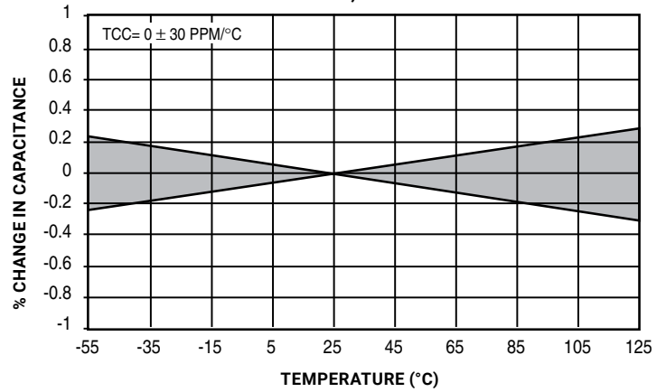
CAPACITANCE CHANGE VS. TEMPERATURE SERIES 700, CASE A
