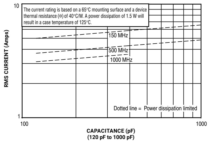
CURRENT RATING VS. CAPACITANCE SERIES 700, CASE A
