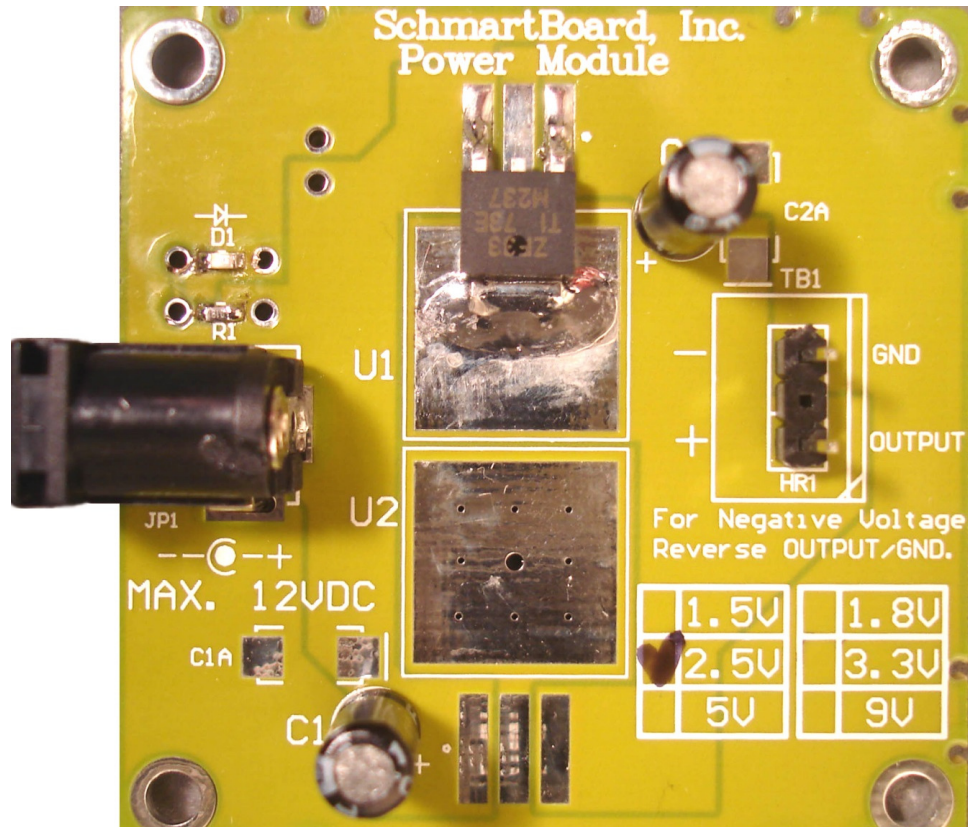
2.5 Volt Populated Single Voltage Regulated Power Module
