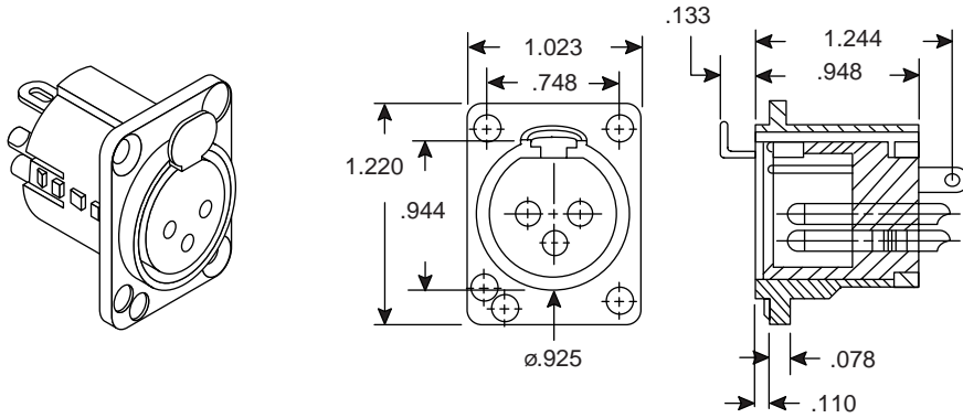
Dimensions (In.)
