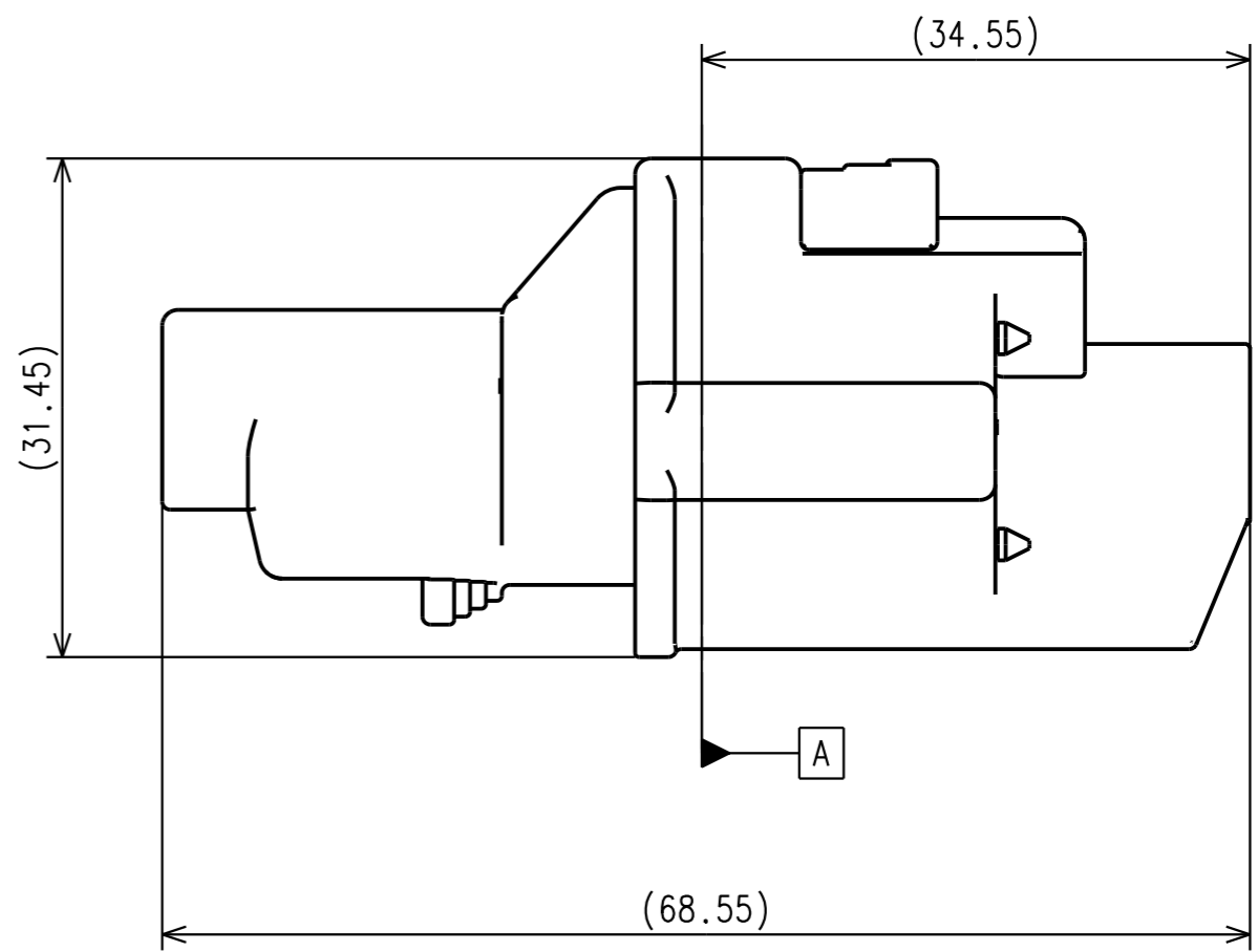
CONNECTOR ASSEMBLY IN FULLY MATED POSITION
