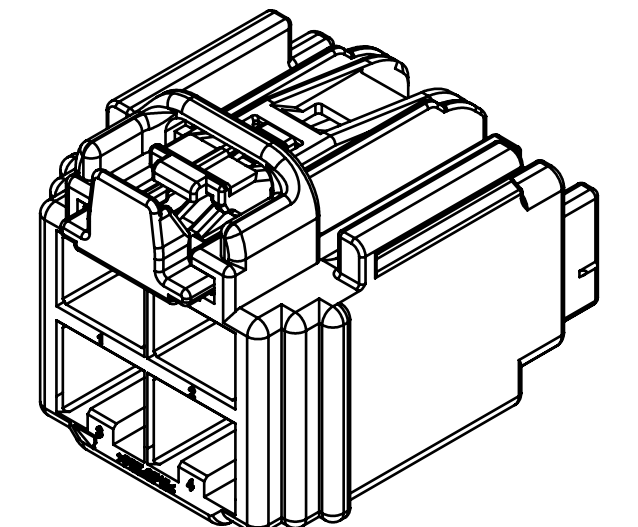
REAR ISOMETRIC VIEW (2/1)
