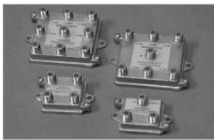
CATV Digital Ready Splitters Vertical, 5 MHz to 1 GHz Features solder sealed back plate providing 130db RF shielding, a printed circuit design that ensures performance up to 1 GHz, and a specially plated Zinc housing and 360° port sealing sleeves allow for excellent corrosion resistance. Port spacing allows for easy installation of security shields, and each comes complete with a
