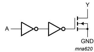
Figure 3. Logic diagram
