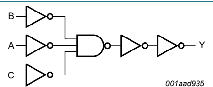
Fig. 3. Logic diagram
