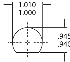
MOUNTING HOLE AE
