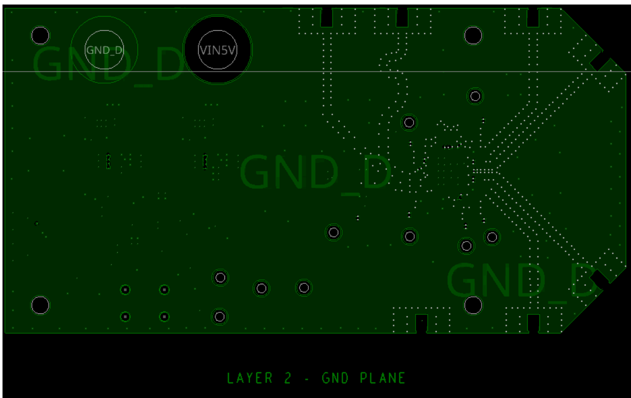
Figure 16. Evaluation Board – Second Layer
