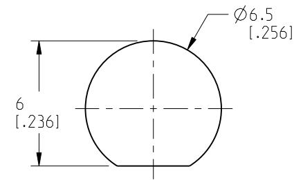
RECOMMENDED MOUNTING HOLE DIMENSIONS
