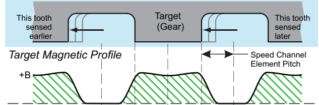
Mechanical Position (Target moves past device pin 1 to pin 2)
