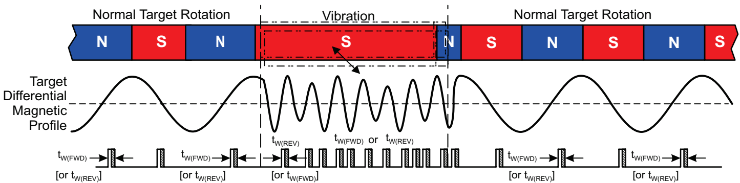
Figure 13: Vibration Behavior
