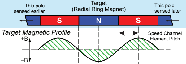
Mechanical Position (Target moves past device pin 1 to pin 2)
