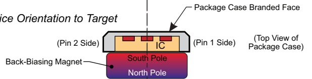
Mechanical Position (Target moves past device pin 1 to pin 2)
