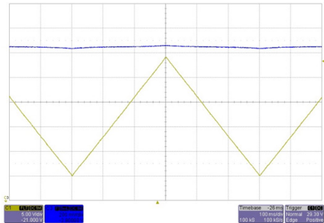
A81805-1 Line Regulation V_{IN} = 8\text{ V} - 30\text{ V} , V_{OUT} = 5\text{ V} I_{OUT} = 2\text{ A}
