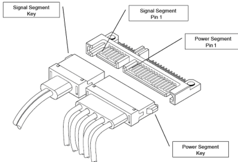
Figure 3-1 SATA Connectors
