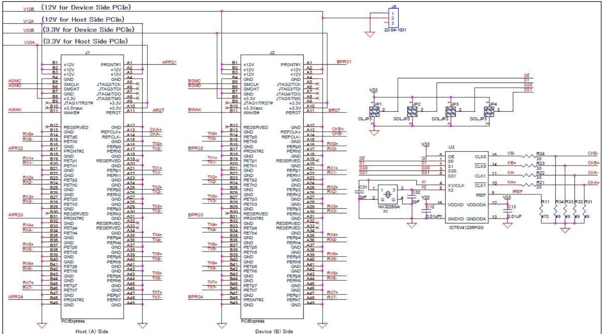
Figure-12: Adapter board schematic (2/2)
