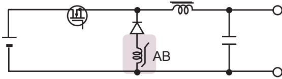
Chopper Converter
