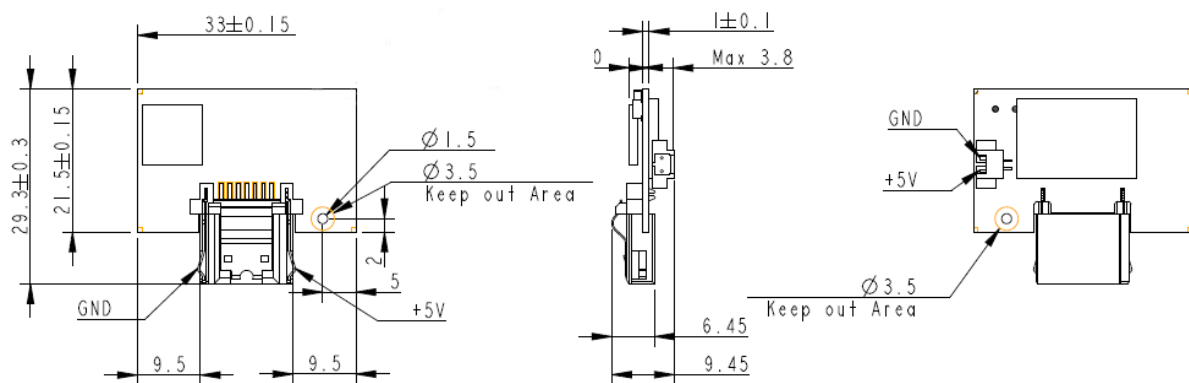
Figure 9-1 Physical Dimensions
