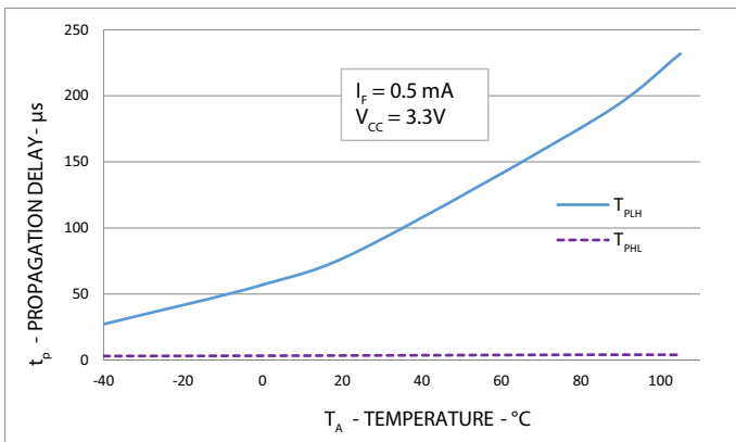
Figure 11: Typical Propagation Delay vs. Temperature
