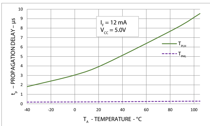
Figure 13: Typical Propagation Delay vs. Temperature
