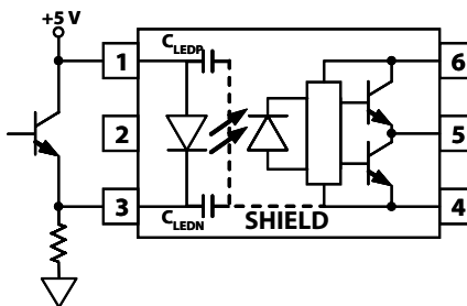
Figure 23 Recommended LED Drive Circuit for Ultra-High CMR Dead Time and Propagation Delay Specifications
