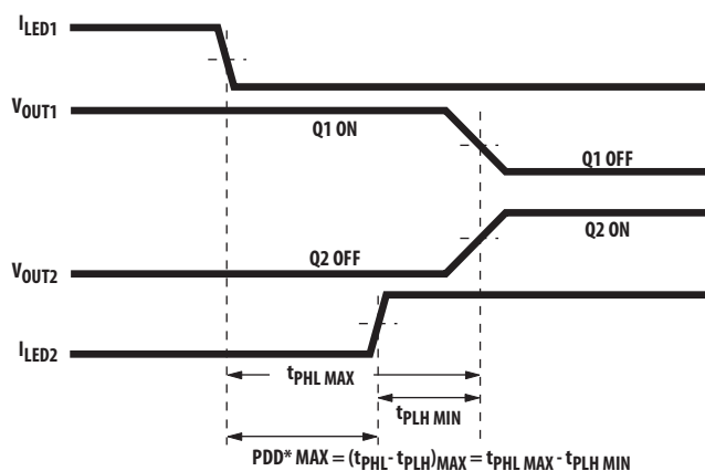
Figure 26 Minimum LED Skew for Zero Dead Time
