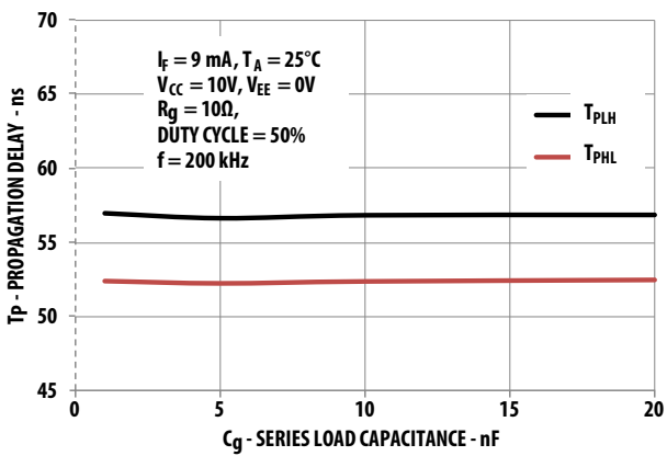
Figure 17: Propagation Delay vs. C_g
