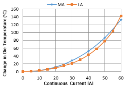
Figure 19: Self heating in the MA and LA package due to current flow
