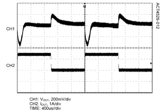
Load Transient (1A-2.4A-1A) V_{in}=12.6V, V_{out}=12V
