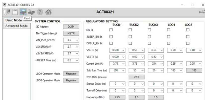
Figure 13 – Read Button
