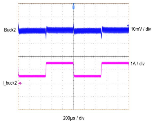
Load Transient Buck2 Vout=0.93V 500mA to 1500mA
