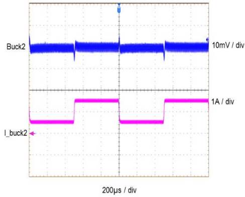
Load Transient Buck2 Vout=0.93V 500mA to 1500mA
