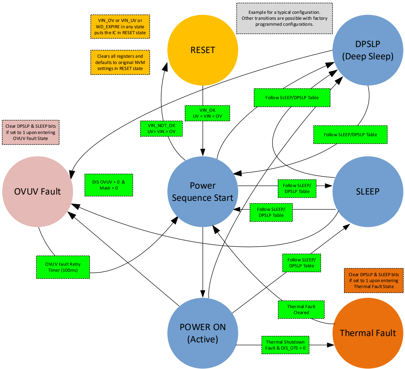
Figure 4: State Machine
