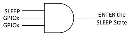
SLEEP State Conditions with SLEEP_MODE = 0
