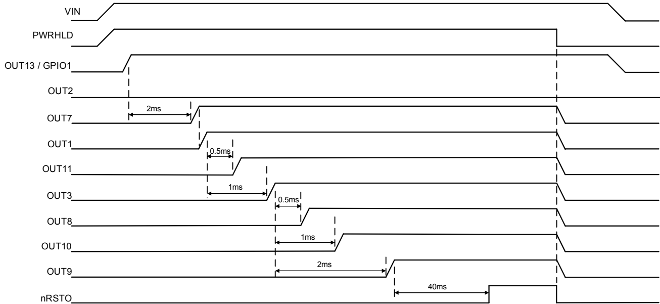
CMI 108 Startup PWREN = 1
