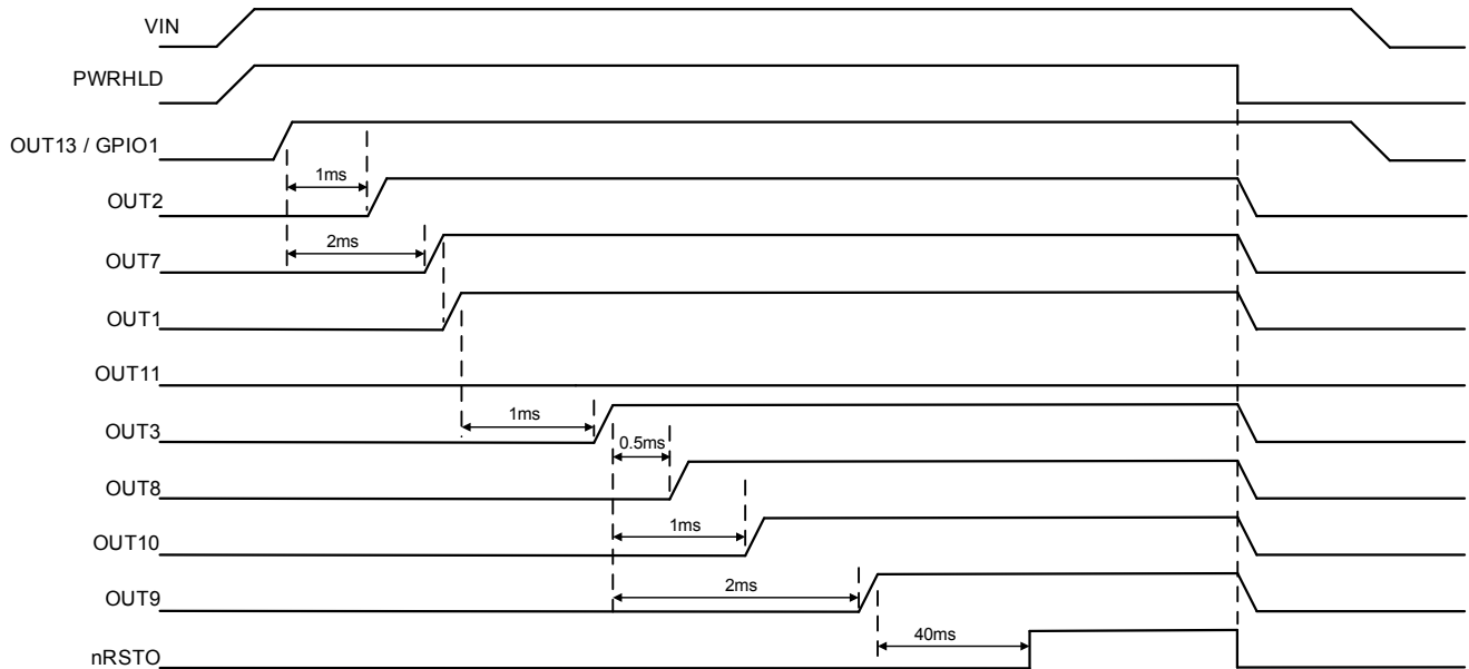
CMI 108 Startup PWREN = 1
