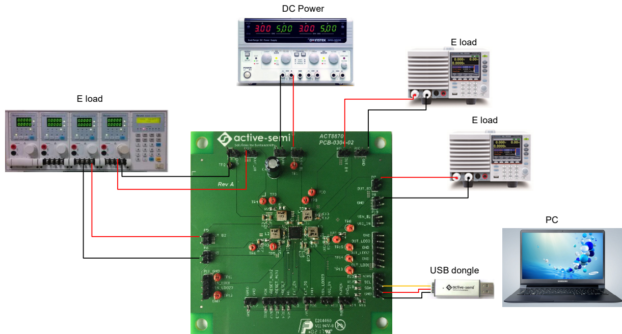
Figure 2 – EVK Setup
