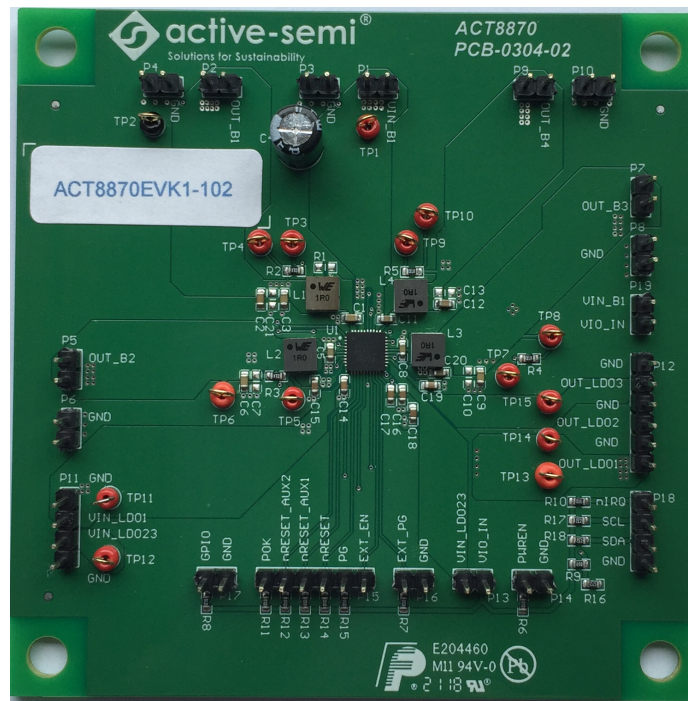
Figure 1 – EVK Picture
