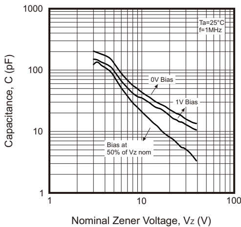
Fig.5 - Typical Capacitance
