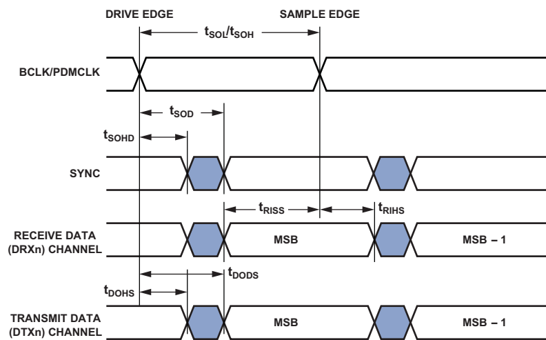
Figure 12. I 2 S Master (A 2 B Subordinate Node) Timing
