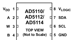
Figure 4. Pin Configuration
