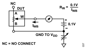
Figure 37. Wiper Resistance
