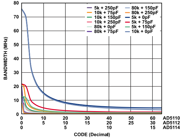
Figure 26. Maximum Bandwidth vs. Code vs. Net Capacitance
