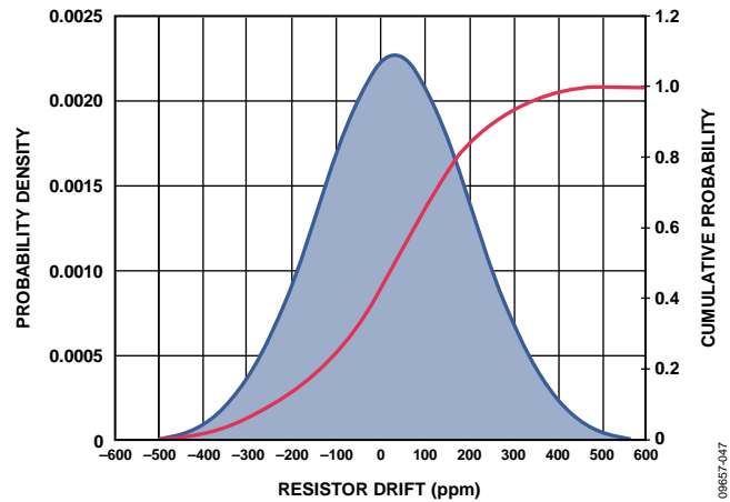
Figure 25. Resistor Lifetime Drift
