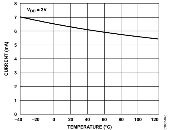
Figure 31. Maximum \overline{A\overline{S\overline{E}}} Output Current vs. Temperature
