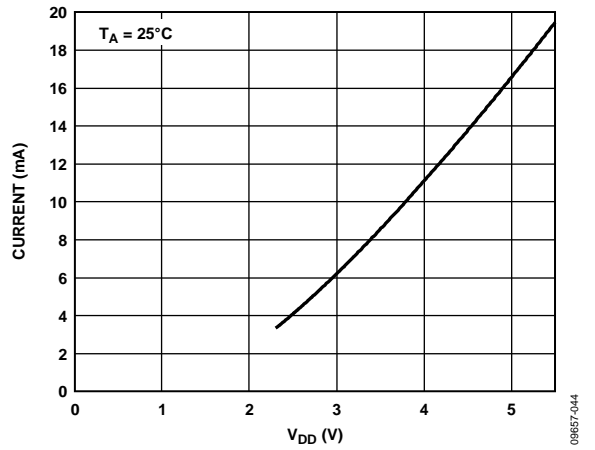
Figure 30. Maximum \overline{A\overline{S\overline{E}}} Output Current vs. Voltage
