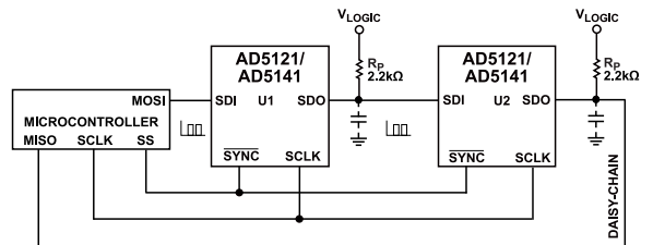
Figure 40. Daisy-Chain Configuration
