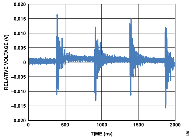
Figure 28. Digital Feedthrough
