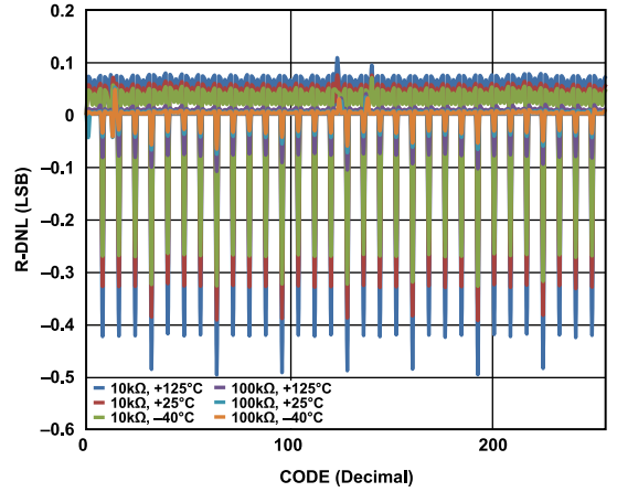
Figure 9. R-DNL vs. Code (AD5142A)
