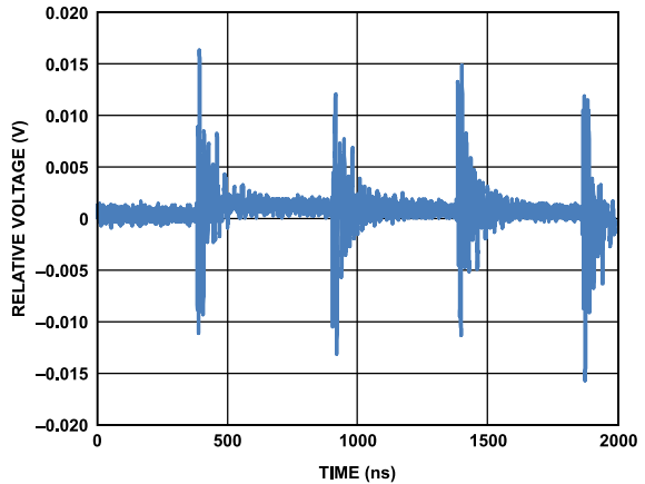
Figure 28. Digital Feedthrough
