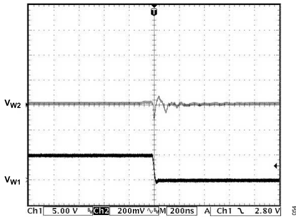
Figure 25. Digital Crosstalk
