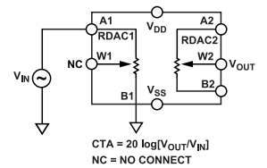
Figure 37. Analog Crosstalk
