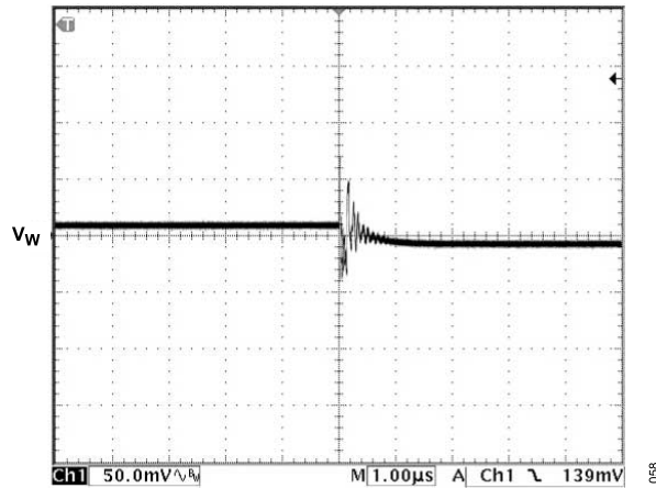
Figure 27. Midscale Glitch, Code 0x80 to Code 0x7F
