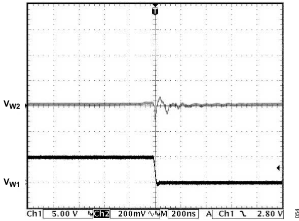
Figure 25. Digital Crosstalk
