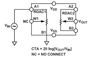
Figure 37. Analog Crosstalk
