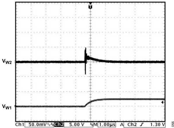
Figure 26. Analog Crosstalk
