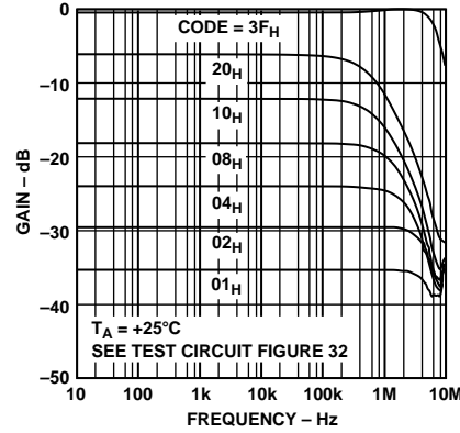
Figure 12. Gain vs. Frequency for R = 10\text{ k}\Omega
