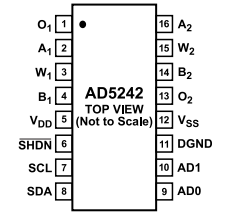
Figure 7. AD5242 Pin Configuration
