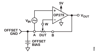
Figure 27. Noninverting Gain
