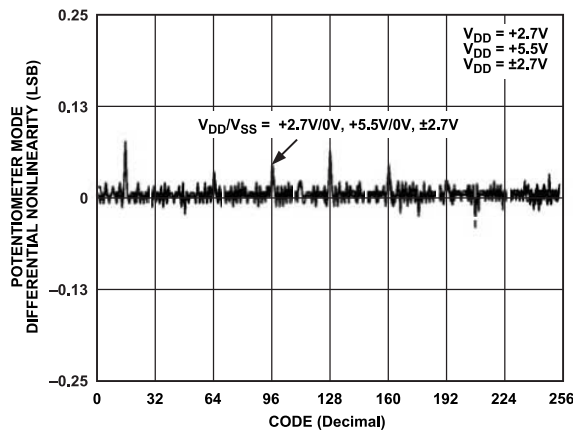
Figure 10. DNL vs. Code
