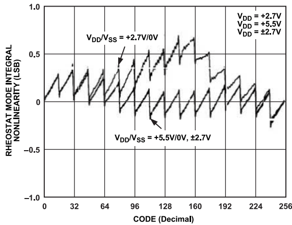
Figure 9. RINL vs. Code
