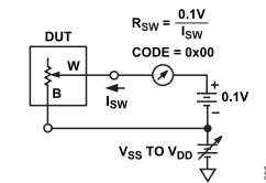
Figure 29. Incremental On Resistance
