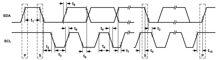
Figure 3. Detail Timing Diagram
