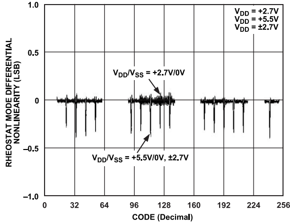
Figure 8. RDNL vs. Code
